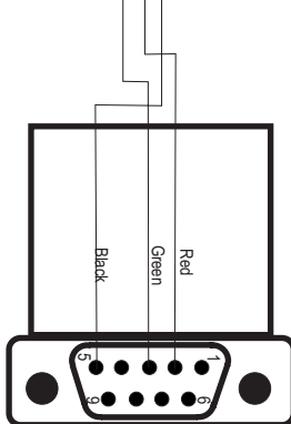
CBLR3PGM, 14 Ft.
