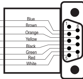
CBLR3MDMFULL, 2 Ft.
