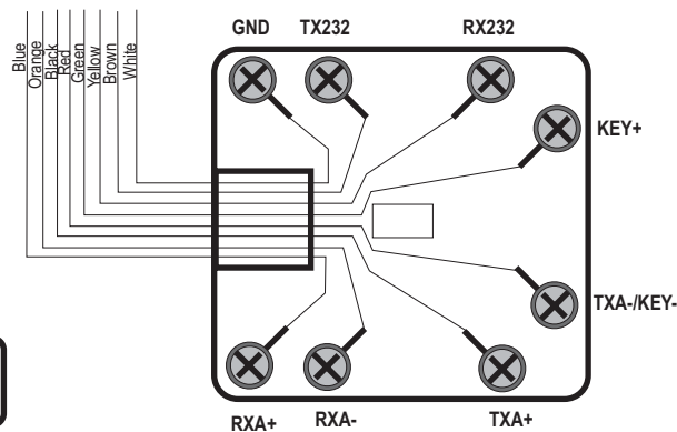
CBLR3SCREWJACK, 2 Ft.
