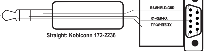
P1 or P2 RS232 Cable, PN R3CBL232
